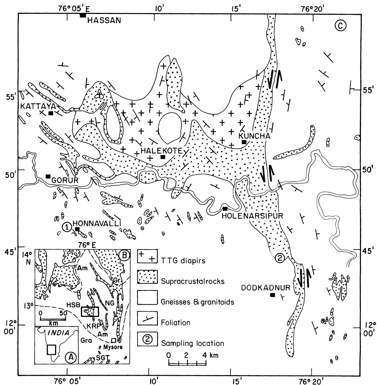
Figure 1. Generalised geological map of the Archean Holenarsipur Supracrustal Belt (HSB) and surrounding gneissic country showing location of the Honnavalli and Dodkadnur meta-anorthosite complexes (based on Hussain and Naqvi 1983). Inset - B shows the location of the HSB in the amphibolite (Am) - facies terrain of the western part of the Dharwar craton, south India which is bounded by greenschist facies (Gr) and Granulite (Gra) facies domains. Other supracrustal belts containing similar stratiform complexes include: Sargur (SG), Nuggihalli (NG) and Krishnarajpet (KRP).
