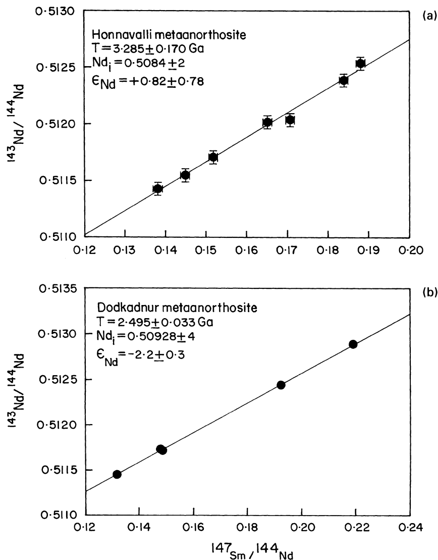
Figure 2. Sm-Nd whole rock isochron diagrams for the Honnavalli and Dodkadnur meta-anorthosite complexes around Holenarsipur.
