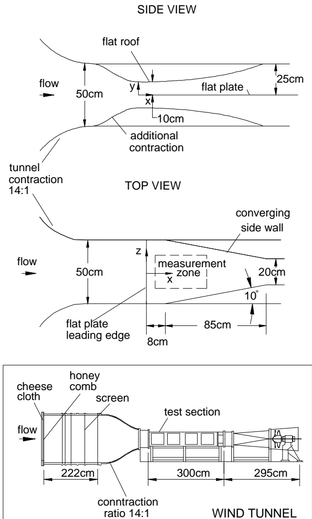
Figure 1. Schematic of the flow geometry.
