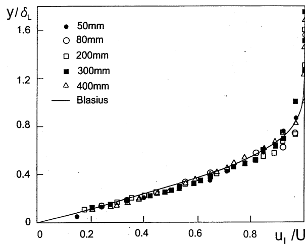
Figure 3. Comparison of the measured laminar velocity profiles with Blasius profile.
