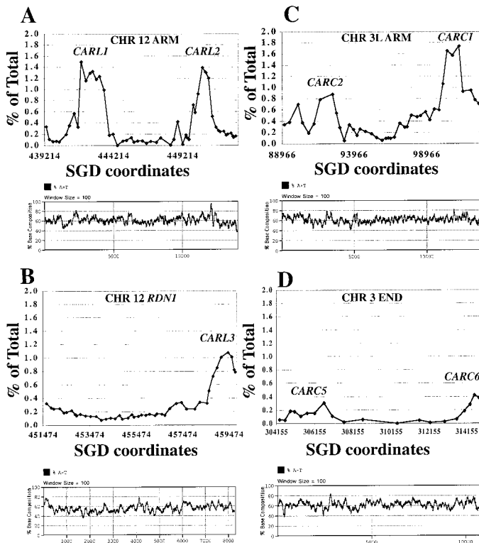
Figure 7. Comparison of characteristics of various Mcd1p-binding sites. AT content of various chromosomal regions aligned with respective Mcd1p-binding profiles. Top graphs are Mcd1p-binding profiles on selected regions of chromosomes XII (left) or 3 (right). Bottom graphs in each set show fluctuations in base composition (AT content on the y axis) revealed by using a sliding window of 100 bp (x axis).
