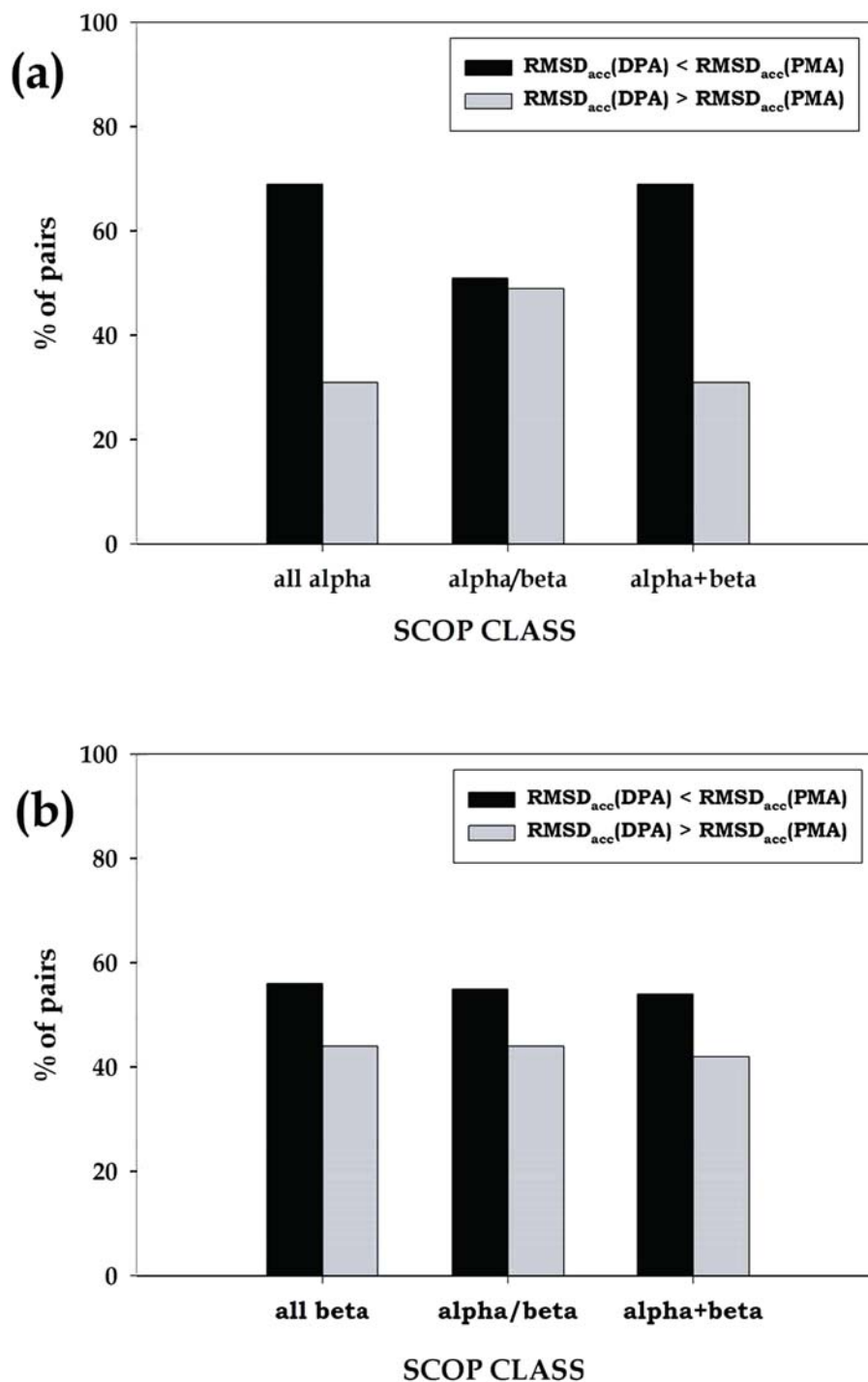
Figure 1. Percentage of pairs of secondary structural elements for various SCOP classes (a) alpha helices (b) beta strands. Number of pairs with better DPA compared to PMA (and viceversa ) as indicated by the RMSD of the solvent accessibilities of the side chains of aligned residues are indicated.
