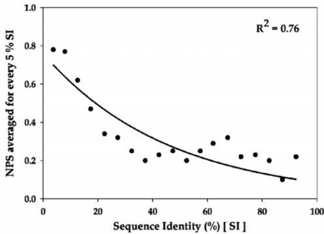
Figure 2. Plot of normalized positional shift between DPA and PMA against sequence identity. Both X and Y-axis parameters are averaged for every 5% of sequence identity.
