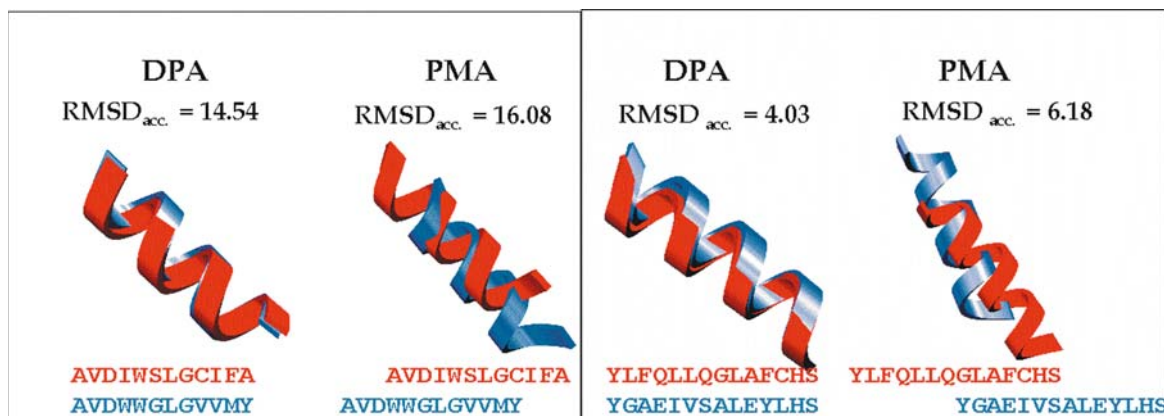
Figure 6. Structural superposition of helices from cyclin-dependent protein kinase (red) with PKB/Akt protein kinase (blue). Root mean square deviation of the side-chain accessibilities of the helices (RMSD acc. ) and the structure dependent sequence alignment blocks from the direct pairwise represented as DPA and pairwise extracted from the multiple structural alignment represented as PMA. This figure and figure 5 have been produced using Setor (Evans, 1993).
