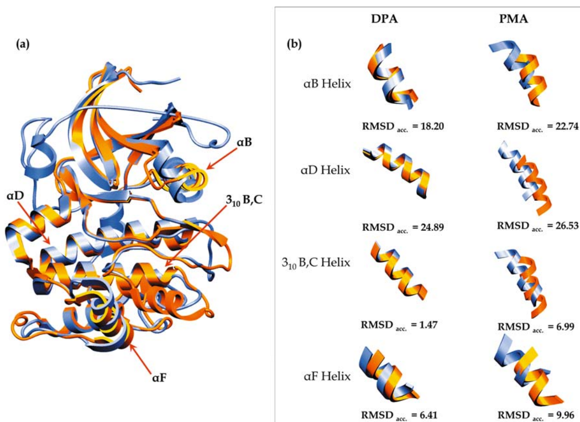
Figure 7. (a) Structural superposition of PKB/Akt protein kinase (blue) and Phosphorylase kinase (orange) with the four helices ( \alpha B, \alpha D, 3_{10} B, C and \alpha F) are marked. (b) The structural superposition of the four helices ( \alpha B, \alpha D, 3_{10} B, C and \alpha F) from the PKB/Akt protein kinase structure with the Phosphorylase kinase structure with the root mean square deviation of the side-chain accessibilities of the respective helices (RMSD acc. ) for the direct pairwise alignment (DPA) and pairwise extracted from the multiple structural alignment (PMA).
