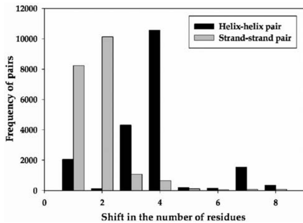
Figure 3. Plot of frequency of helix-helix and strand-strand alignment segments against shift in the alignment positions between DPA and PMA.
