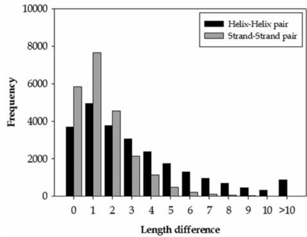
Figure 4. Plot of frequency of helix-helix and strand-strand alignment segments against the length difference between the segments.
