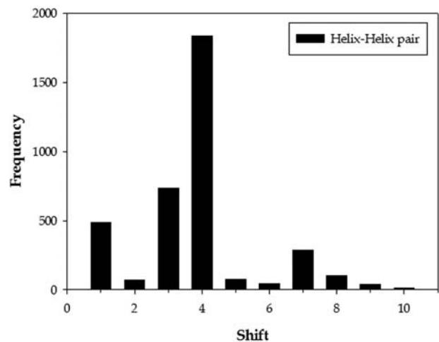
Figure 5. Plot of frequency of helix-helix alignment segments with zero length difference against the shift in the alignment positions between DPA and PMA.
