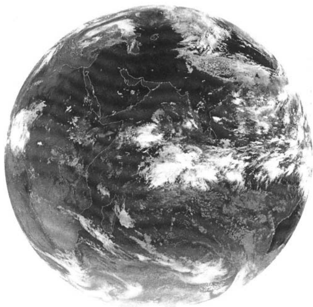
Figure 1. Brightness temperature in the infrared channel from METEOSAT on 15 June 2006 showing the Inter-Tropical Convergence Zone just below the equator (courtesy: http://www.sat.dundee.ac.uk ).
