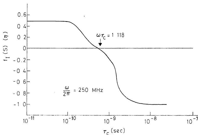
Figure 12. Dependence of ^1H - ^1H NOE magnitude ( \eta ) on the correlation time \tau_c (from Balaram et al 1973).
