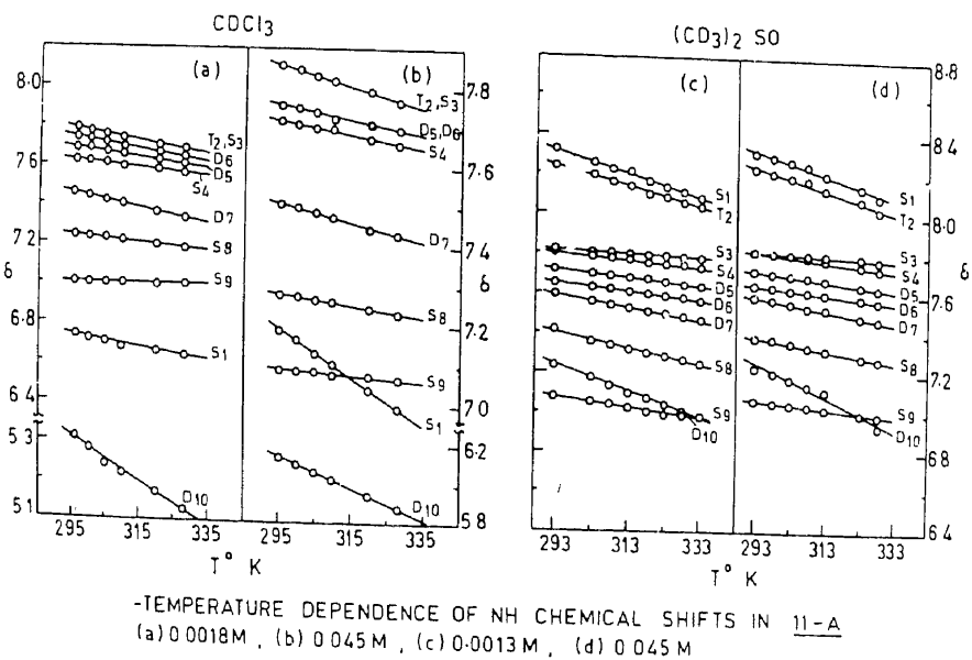
Figure 10. Temperature dependence of NH chemical shifts in the peptide Boc-Ala-Aib-Leu-Aib-Gly-Leu-Aib-Pro-Val-Aib-Aib-OMe ( 11A ). (a) \text{CDCl}_3 , 0.0018 M peptide. (b) \text{CDCl}_3 0.045 M. (c) (\text{CD}_3)_2\text{SO} , 0.0013 M. (d) (\text{CD}_3)_2\text{SO} , 0.045 M.
