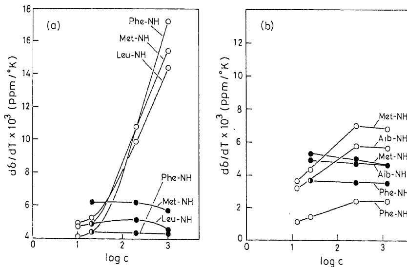
Figure 7. Concentration dependence of temperature coefficients ( d\delta/dT ) of NH resonances in chemotactic peptide analogs. (a) Formyl-Met-Leu-Phe-OMe • (\text{CD}_3)_2\text{SO} ; o \text{CDCl}_3 (b) Formyl-Met-Aib-Phe-OMe • (\text{CD}_3)_2\text{SO} ; o \text{CDCl}_3 -Abscissa defined as in figure 6 (from Raj and Balaram 1985).
