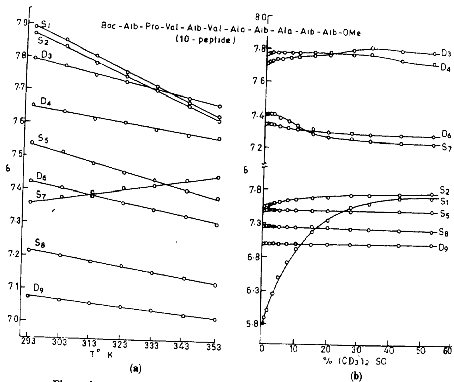
Figure 4. (a) Temperature dependence of NH chemical shifts in the decapeptide Boc-Aib-Pro-Val-Aib-Val-Ala-Aib-Ala-Aib-Aib-OMe in (CD_3)_2SO . S_n , D_n refer to singlet and doublet NH resonances. The subscript n refers to the order of appearance from low field in (CD_3)_2SO . (b) Dependence of NH chemical shifts on solvent composition in CDCl_3 - (CD_3)_2SO mixtures (from Iqbal and Balaram 1981a).
