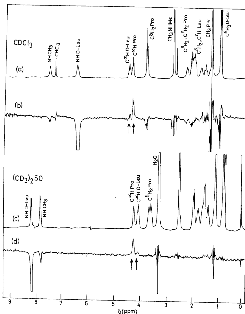
Figure 13. 270 MHz ^1\text{H} NMR spectra of Pivaloyl-Pro-D-Leu-NHMe in (a) \text{CDCl}_3 and (c) (\text{CD}_3)_2\text{SO} . (b) Difference NOE spectrum ( \times 16 ) in \text{CDCl}_3 on saturation of D-Leu NH. Note partial saturation of \text{NHCH}_3 . (d) Difference NOE spectrum ( \times 4 ), in (\text{CD}_3)_2\text{SO} on saturation of D-Leu NH. Note partial saturation of \text{NHCH}_3 . Arrows indicate observed NOE's (from Balaram 1984).
