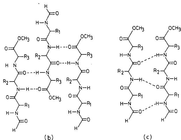
Figure 8. Schematic representation of aggregation modes for Formyl-Met-Leu-Phe-OMe in chloroform, consistent with NMR data. (a) antiparallel \beta -sheets 'in register'. (b) antiparallel \beta -sheets 'out register'. (c) parallel \beta -sheet aggregates.
