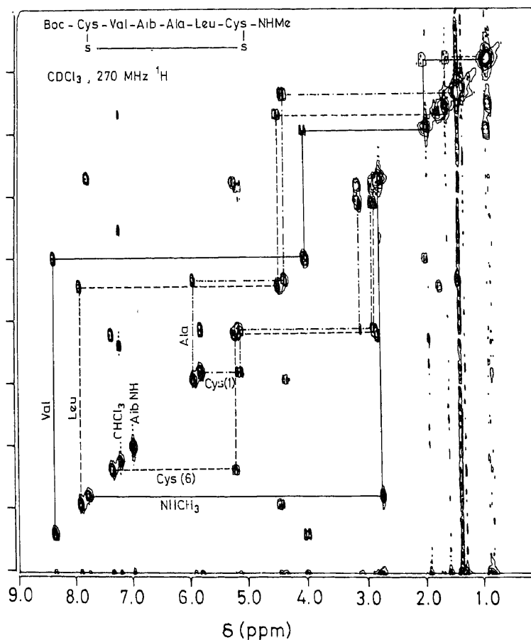
Figure 1. 270 MHz ^1H cosy spectrum (contour plot) of the peptide Boc-Cys-Val-Aib-Ala-Leu-Cys-NHMe in CDCl 3 . Connectivities of NH-C^{\alpha}-H-C^{\beta}H_2 protons
