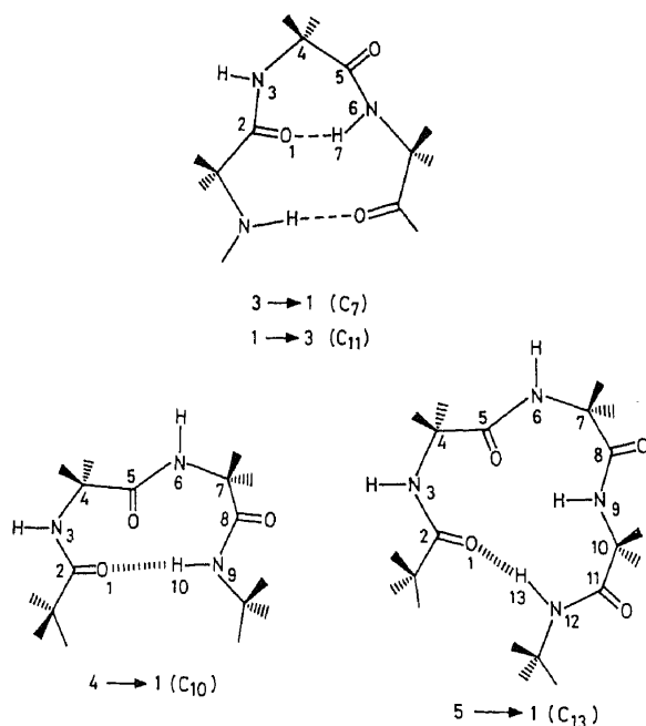
Figure 3. Representative intramolecularly hydrogen bonded conformations in peptides.
