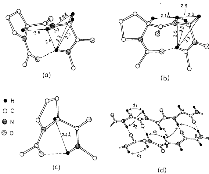
Figure 11. Interproton distances in idealized peptide conformations. (a) Pro-Gly type I \beta -turn. (b) Pro-Gly type II \beta -turn. (c) \gamma -turn ( C_7 ) conformation. (d) Antiparallel \beta -sheet conformation. d_1 ( C_iH-N_{i+1}-H ) is generally 2.2–2.4 Å and gives rise to large NOEs. d_2 and d_3 are generally \geq 3.0 Å in this structure. Transannular NOEs are weak but observable (Kuo and Gibbons 1980; Billeter et al 1982; Wagner et al 1981).
