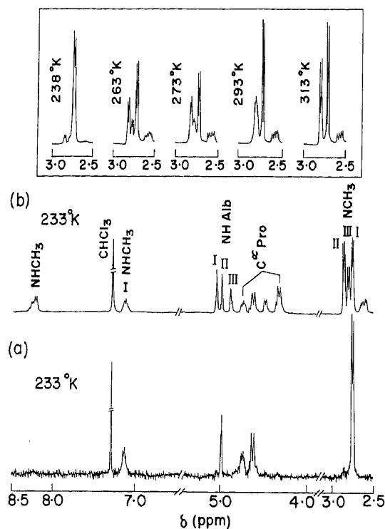
Figure 17. (a) Low temperature 270 MHz ^1\text{H} NMR spectrum of single crystals of Boc-Aib-Pro-Pro-NHMe recorded immediately after dissolution in \text{CDCl}_3 , pre-cooled in liquid \text{N}_2 and transferred to the probe at 233 K. (b) Low temperature 270 MHz ^1\text{H} NMR spectrum of a noncrystalline sample of Boc-Aib-Pro-Pro-NHMe at 233 K in \text{CDCl}_3 . (Inset) Methylamide \text{CH}_3 resonances (doublets) in Boc-Aib-Pro-Pro-NHMe. The sample was prepared as in (a) and the spectra recorded at various temperatures. I, II, III indicate an assignment to the Pro-Pro conformers described in figure 16 (from Balaram et al 1983).
