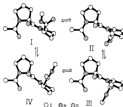
Figure 16. Perspective view of the low energy conformations of a Pro-Pro sequence. Calculations were performed on the model Ac-Pro-Pro-NHMe. I ( trans-trans' ); II ( cis-trans' ); III ( cis-cis' ); IV ( trans-cis' ). Trans and cis refer to the \omega = 180^\circ and \omega = 0^\circ conformations about the Pro-Pro bond, respectively. Trans' and cis' refer to conformations in the region \psi \sim 130^\circ and \psi \sim -50^\circ , respectively for the first Pro residue (from Balaram et al 1983).
