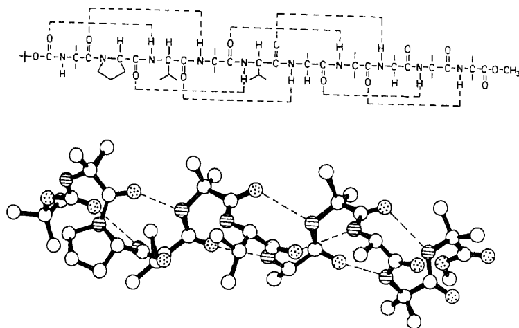
Figure 5. (bottom) Solid state conformation of Boc-Aib-Pro-Val-Aib-Val-Ala-Aib-Ala-Aib-Aib-OMe determined by x-ray diffraction (Francis et al 1983). Note 3_{10} -helical (4 \rightarrow 1) hydrogen bonding pattern. (top) Intramolecular hydrogen bonding scheme proposed on the basis of ^1H NMR studies (Iqbal and Balaram 1981a).
