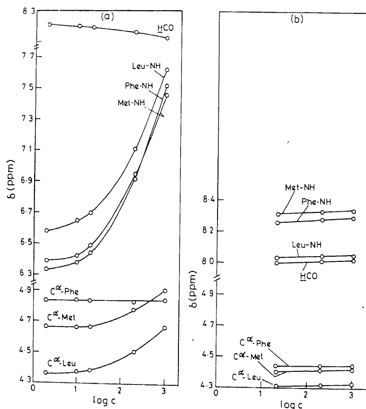
Figure 6. Concentration dependence of chemical shifts ( \delta ) for various resonances in Formyl-Met-Leu-Phe-OMe in \text{CDCl}_3 (a) and (\text{CD}_3)_2\text{SO} (b). Abscissa expresses concentration as \log c , where c = molar concentration of peptide \times 10^4 (from Raj and Balaram 1985).
