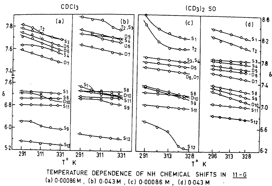
Figure 9. Temperature dependence of NH chemical shifts in the suzukacillin 7-17 fragment Boc-Gln-Aib-Leu-Aib-Gly-Leu-Aib-Pro-Val-Aib-Aib-OMe ( 11G ). (a) \text{CDCl}_3 , 0.00086 M peptide. (b) \text{CDCl}_3 , 0.043 M. (c) (\text{CD}_3)_2\text{SO} 0.00086 M. (d) (\text{CD}_3)_2\text{SO} 0.043 M.
