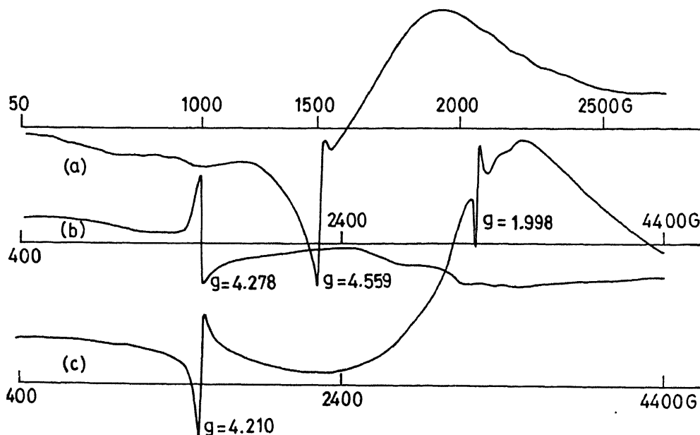
Figure 2. EPR spectra of a plagioclase from Holenarasipur (frequency, 9.2 GHz; temperature 78 K. (a) Untreated sample, (b) Oxidized at 650°C, (c) reduced at 650°C.
