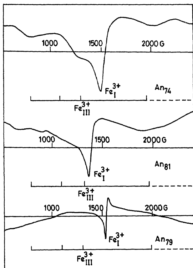
Figure 1. Typical EPR spectra for \text{Fe}^{3+} in plagioclases from Holenarasipur anorthosites (February, 9.2 GHz; temperature, 78 K).
