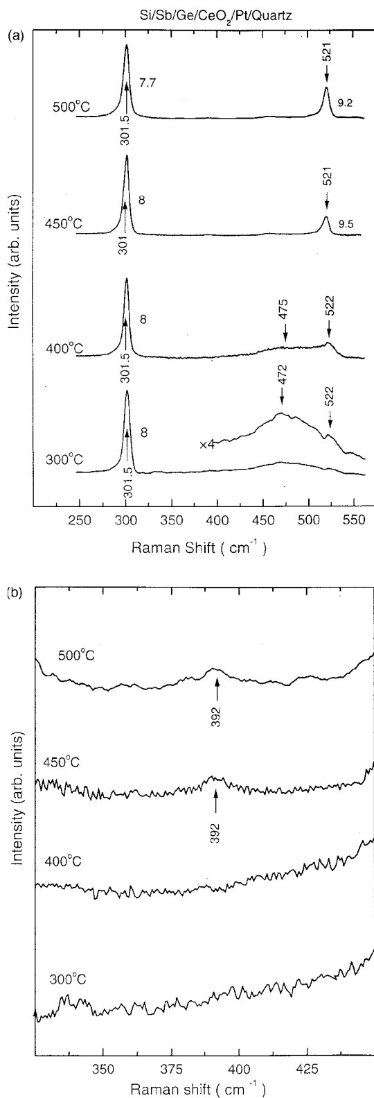
FIG. 4. (a) IERS spectra of Si on Ge grown with Sb as surfactant. The numbers near the peaks state their FWHM. (b) Figure 4(a) expanded in X and Y scale.
