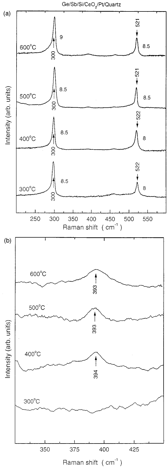
FIG. 2. (a) IERS spectra of Ge grown on Si with Sb as surfactant. The numbers near the peaks state their FWHM. (b) Figure 2(a) expanded in X and Y scales.
